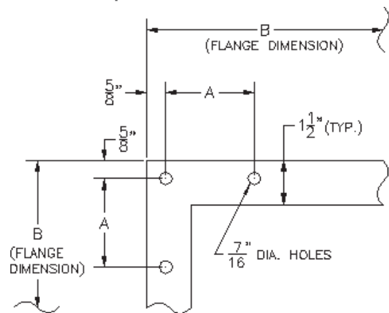
Isolation Damper Bolt Hole Patterns
